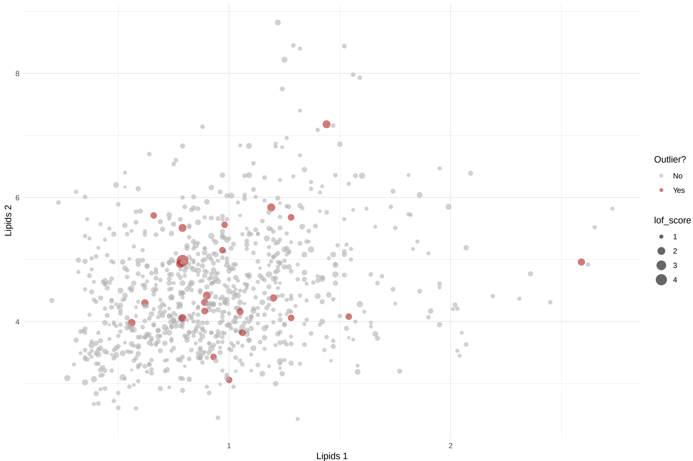
Bivariate Scatterplot with LOF Outliers Red points represent multivariate outliers (LOF > 1.5)
